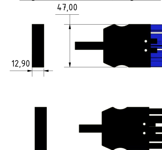
WAGO Winsta Midi 771 MALE connector
